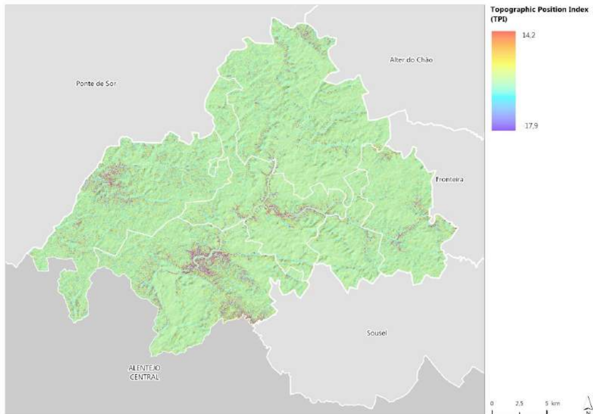
Figura 42. Topographic Position Index (TPI) 47
